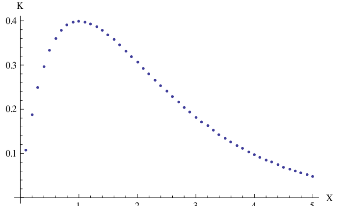
Fig. 4. (Color online) Computed results for |K(X)| given by equation (11).
