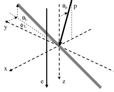
Fig. 3. Depiction of the cylindrical scattering geometry more likely in practical cases.
