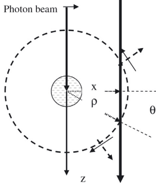
Fig. 2. Illumination arrangement and coordinate set up assumed for the illustrative calculation of photon-electron interaction near a cylinder.
