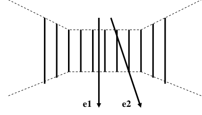
Fig. 1. Schematic diagram of electron beam paths near the antinodes in a standing light wave. Such a phase shifting device, placed in the back-focal plane, would not intercept the waves scattered by the object but only the unscattered wave. For aligned paths such as e1, the periodic optical potential would generate Kapitza-Dirac diffraction but this effect would be averaged out for trajectories like e2.
